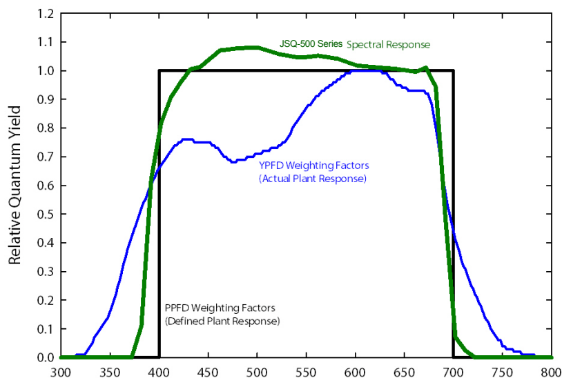
Radiation weighting factors for PPFD (black line, defined plant response to radiation), YPFD (blue line, measured plant response to radiation), and Apogee JSQ-500 Series Quantum Sensors (green line, sensor sensitivity to different wavelengths of radiation).
